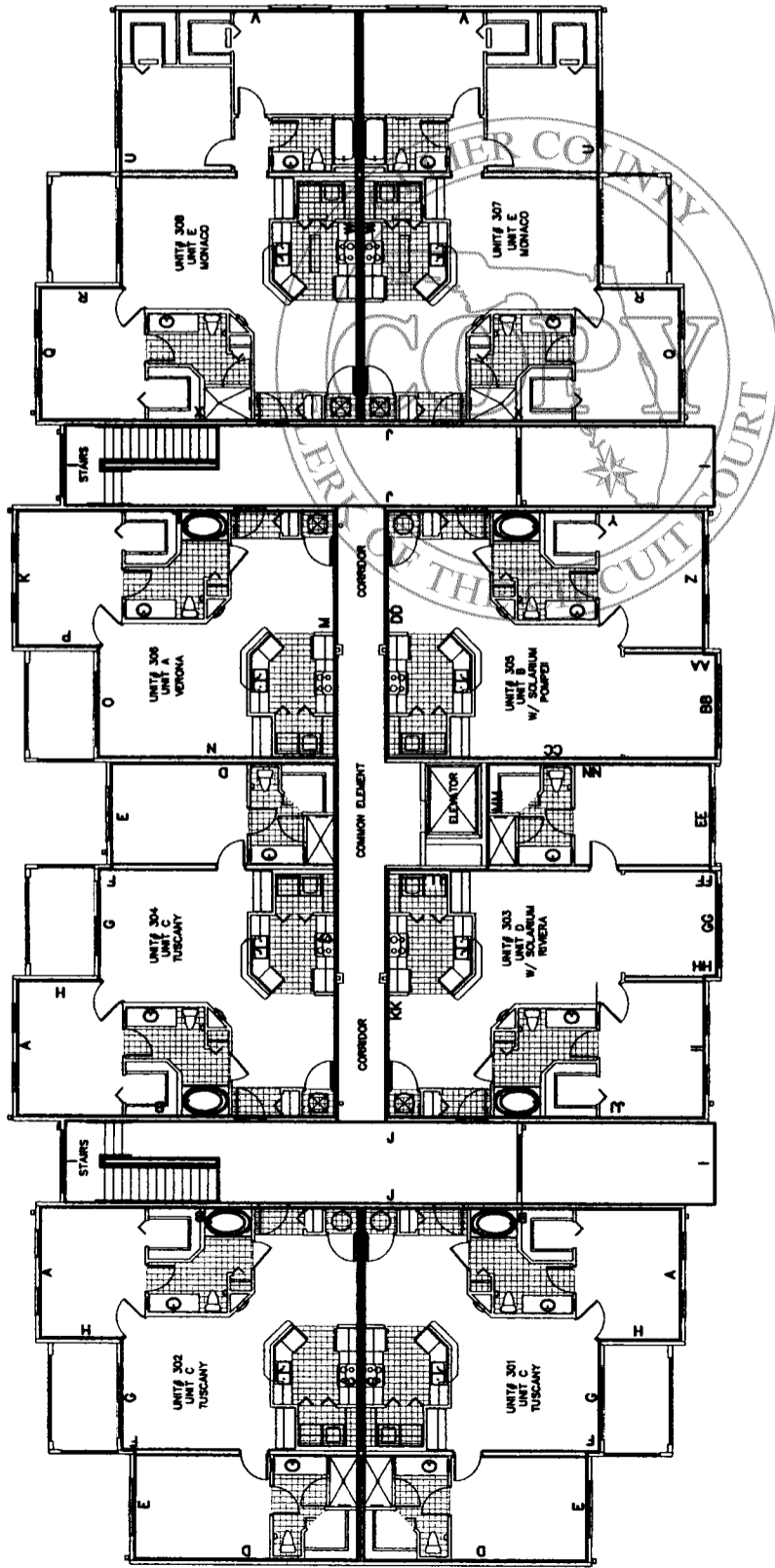
FLOOR PLAN - BUILDING TYPE 1 - THIRD FLOOR
